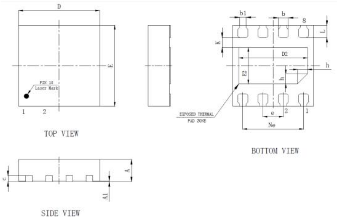
DFN8L-2×2
